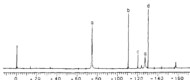
Figure 4. ^{19}\text{F} NMR spectrum of a \text{CDCl}_3 solution of the reaction product of \text{Mes}_2\text{SiF}_2 with \text{Et}_4\text{NF}\cdot 2\text{H}_2\text{O} in the presence of DMP in acetonitrile solution. The products formed at 25^\circ\text{C} are (a) [\text{Mes}_2\text{SiF}_3]^- (\text{F}_{\text{ax}}) , (b) [\text{MesSiF}_4]^- , (c) \text{Mes}_2\text{Si}(\text{F})\text{-O-Si}(\text{F})\text{Mes}_2 , (d) [\text{Mes}_2\text{SiF}_3]^- (\text{F}_{\text{eq}}) , and (e) [\text{Mes}_2\text{Si}(\text{F})\text{O-H-O-Si}(\text{F})\text{Mes}_2]^- . The small signal at -123.8 ppm is due to unreacted \text{Mes}_2\text{SiF}_2 , while the small signal at -157.6 ppm is unassigned.
