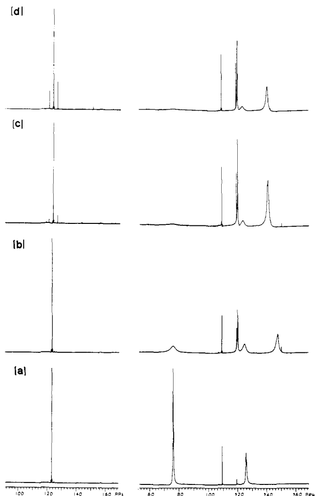
Figure 5. The left side shows ^{19}\text{F} NMR spectra at 25 °C of (a) an acetone solution of \text{Me}_2\text{SiF}_2 ; (b) the solution in (a) to which water was added to give a 2:1 molar ratio of water to \text{Me}_2\text{SiF}_2 recorded after 5 min of mixing; (c) the solution of (b) after 15 min, and (d) the solution in (b) after 24 h. The right side shows an identical time sequence and molar solution concentrations of the ^{19}\text{F} NMR spectra at 25 °C of an acetone solution of [\text{Me}_2\text{SiF}_3][\text{K},18\text{-c-}6] . Proceeding from low to high field, the ^{19}\text{F} signals in (b)–(d) arise from [\text{Me}_2\text{SiF}_3]^- ( F_{ax} ) at -76.04 ppm, [\text{MesSiF}_4]^- at -109.26 ppm, [\text{Mes}_2\text{Si}(\text{F})\text{O-H-O-Si}(\text{F})\text{Mes}_2]^- at -119.24 ppm, \text{Mes}_2\text{Si}(\text{F})\text{-O-Si}(\text{F})\text{Mes}_2 at -120.1 ppm, [\text{Me}_2\text{SiF}_3]^- ( F_{eq} ) at -125.81 ppm, and an unidentified peak which varies between -148 and -140 ppm.
