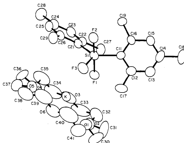
Figure 1. ORTEP plot of the anion and cation in [\text{Mes}_2\text{SiF}_3][\text{K},18\text{-c-6}]\cdot\text{CH}_2\text{Cl}_2 (1) with thermal ellipsoids at the 30% probability level. Hydrogen atoms are omitted for purposes of clarity.
