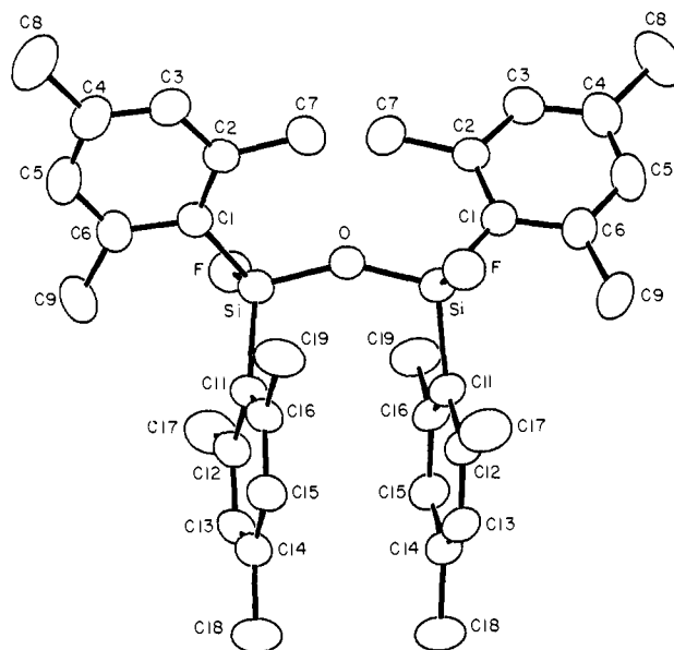
Figure 3. ORTEP plot of (\text{Mes}_2\text{SiF})_2\text{O} ( 3 ) with thermal ellipsoids at the 30% probability level. Atoms on the right of the figure are 2-fold related ( 1-x, y, 1.5-z ) to those on the left with the same label. The oxygen atom lies on the 2-fold axis. Hydrogen atoms are omitted for purposes of clarity.
